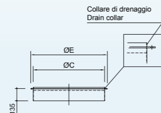
ANELLO SOTTOFILTRO A SALDARE FILTER MOUNTING UPSTAND
